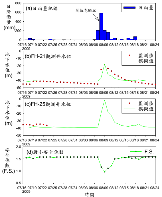
圖 7 吉露調查範圍降雨誘發崩塌潛勢評估分析成果 Fig.7 Analysis results of rainfall-induced Ji-Lou landslide hazard assessment
